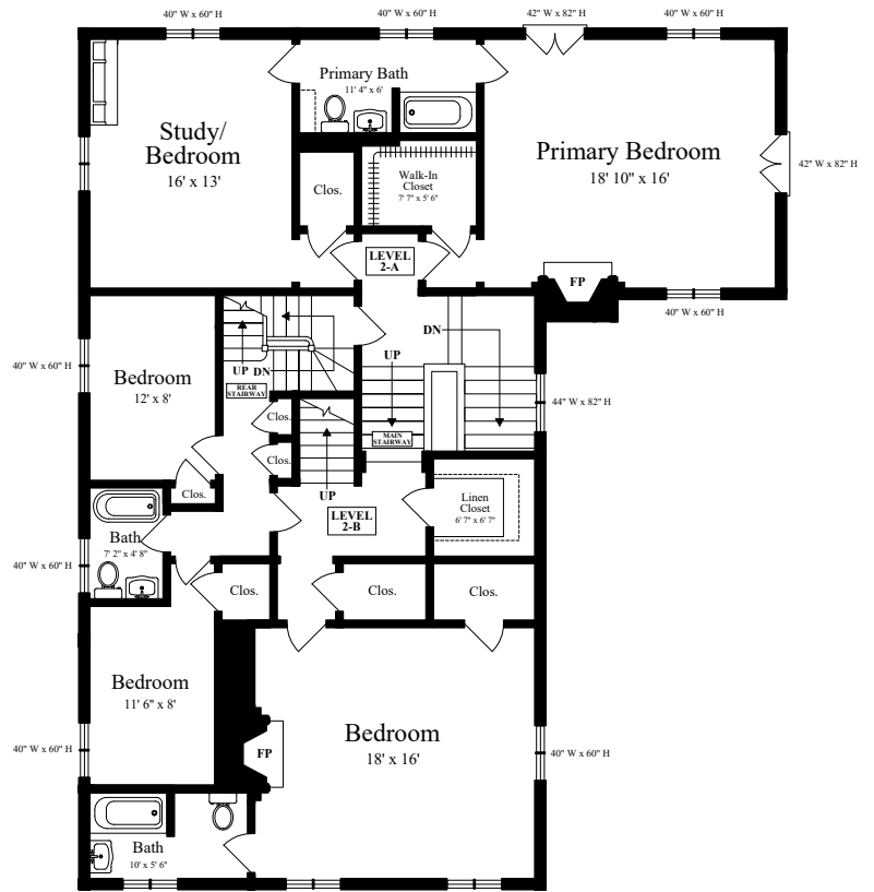
SECOND LEVELS (ceiling = 8')
